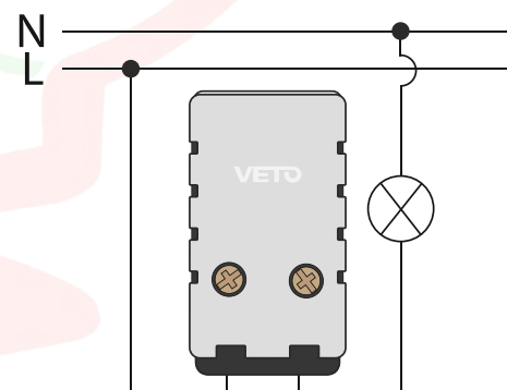
Dimmer simple
